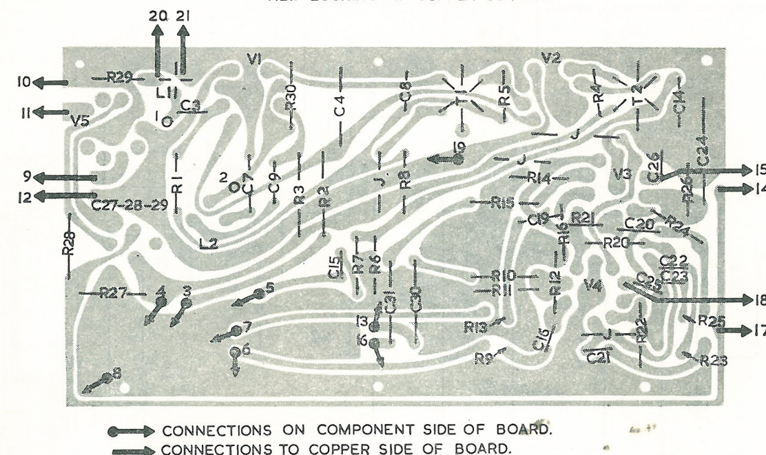
PRINTED BOARD LAYOUT AND CONNECTIONS. VIEW LOOKING AT COPPER SURFACE.
