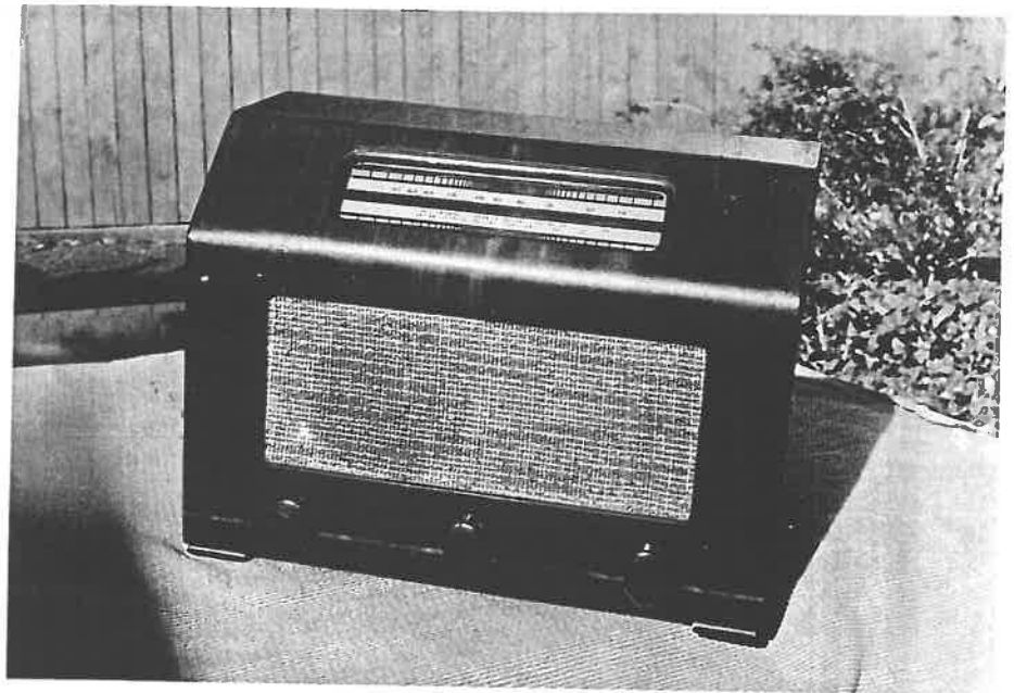
Pacific 5-tube B.C. Model 576 1946
