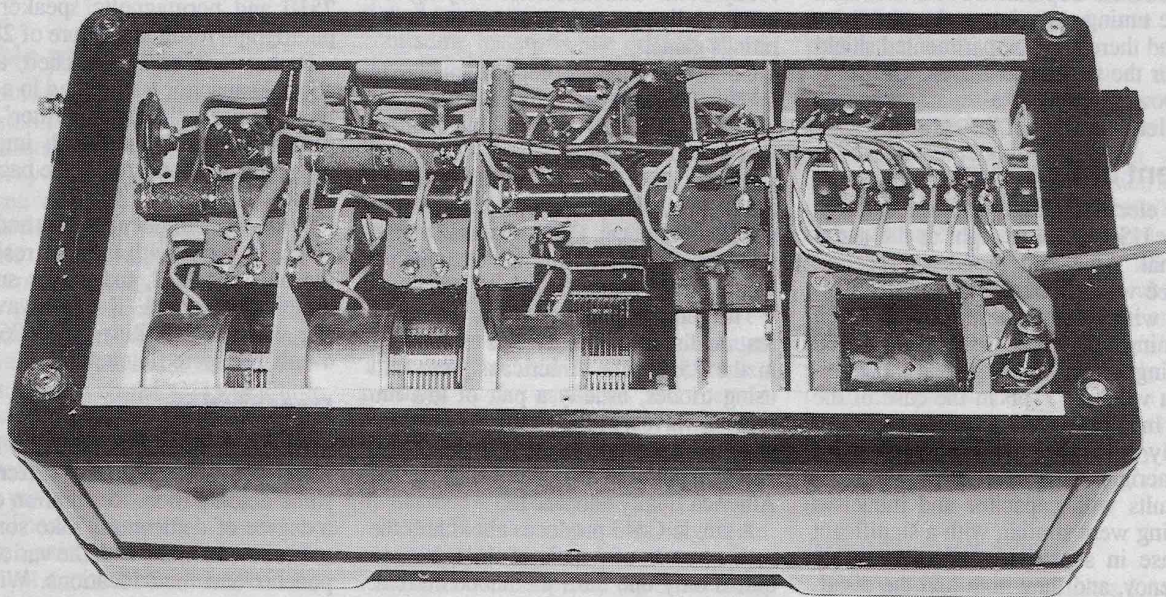
Fig.4: With the bottom panel removed, most of the wiring and components are accessible.
