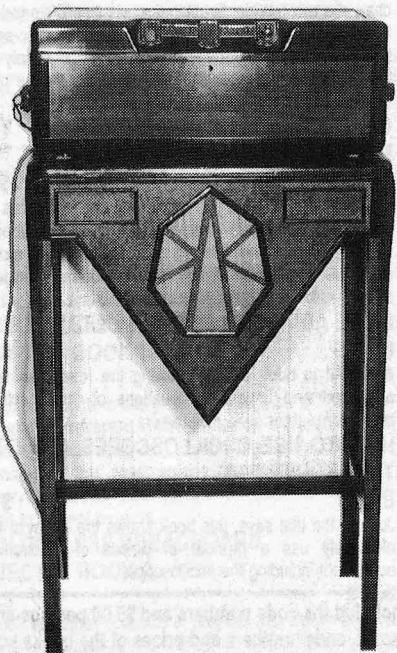
Fig.1 (right): The 2510 was very popular when combined as shown here with the 'Sevenette' magnetic (moving iron) speaker.
