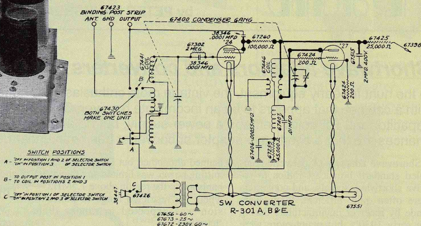
Fig.3: In 1931, Stewart Warner brought out its R301 converter, originally in a small pagoda-topped cabinet. The valve filaments are run from its own transformer.
