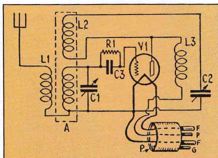
Fig.1 (above): The earliest 'add ons' for shortwave reception were simple regenerative grid-leak detector units plugged into the detector socket of a broadcast receiver. In this 1929 design, C2 is the regeneration control and L3 an RF choke.
