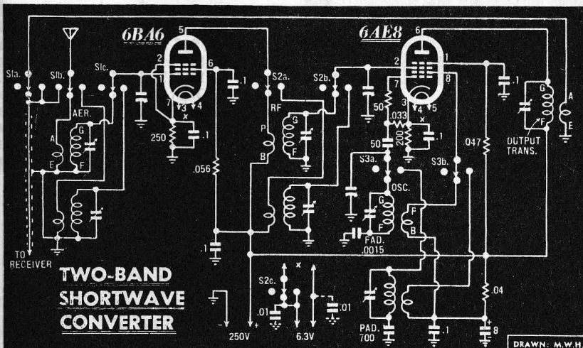
Fig.6: This two-band converter was a July 1955 R,TV&H project, incorporating an RF stage and high gain miniature valves. When coupled into a typical domestic receiver, performance would have been superior to anything short of a communications receiver. A connection of the receiver's AGC line to the grid circuit of the 6BA6 RF amplifier would have been a worthwhile refinement.
