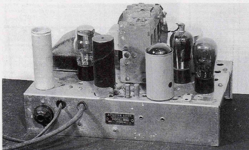
Fig.4: Far from being experimenter's inexpensive add-ons, some converters were very well made and intended to be integrated with the manufacturer's receivers. With its own power supply and an IF amplifier, and using the standard Atwater Kent nickel plated mantel receiver chassis, the self-contained four valve Atwater Kent 1932 three-band model 93 was as complex and cost as much as some complete receivers. It could be used as a stand for the model 567 (right).
