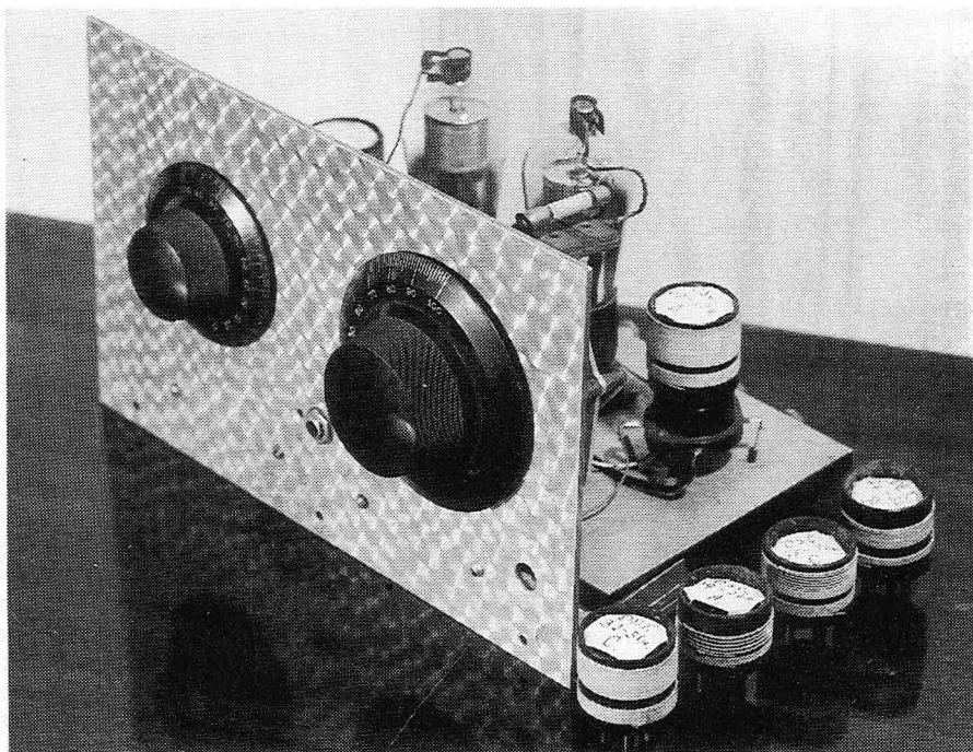
Fig.1 (above): The earliest 'add ons' for shortwave reception were simple regenerative grid-leak detector units plugged into the detector socket of a broadcast receiver. In this 1929 design, C2 is the regeneration control and L3 an RF choke.
