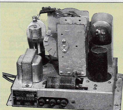
Fig.3: In 1931, Stewart Warner brought out its R301 converter, originally in a small pagoda-topped cabinet. The valve filaments are run from its own transformer.
