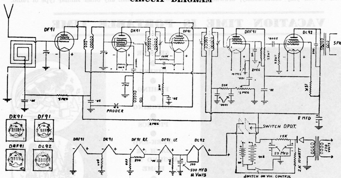
CIRCUIT DIAGRAM
