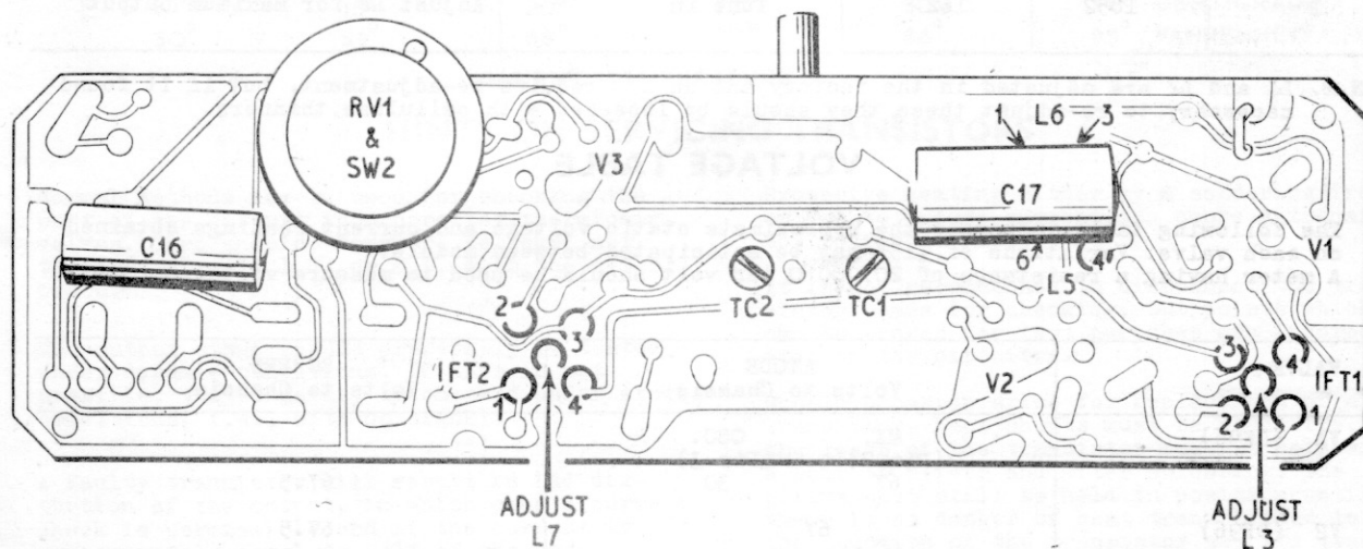
UNDERSIDE VIEW OF CHASSIS
