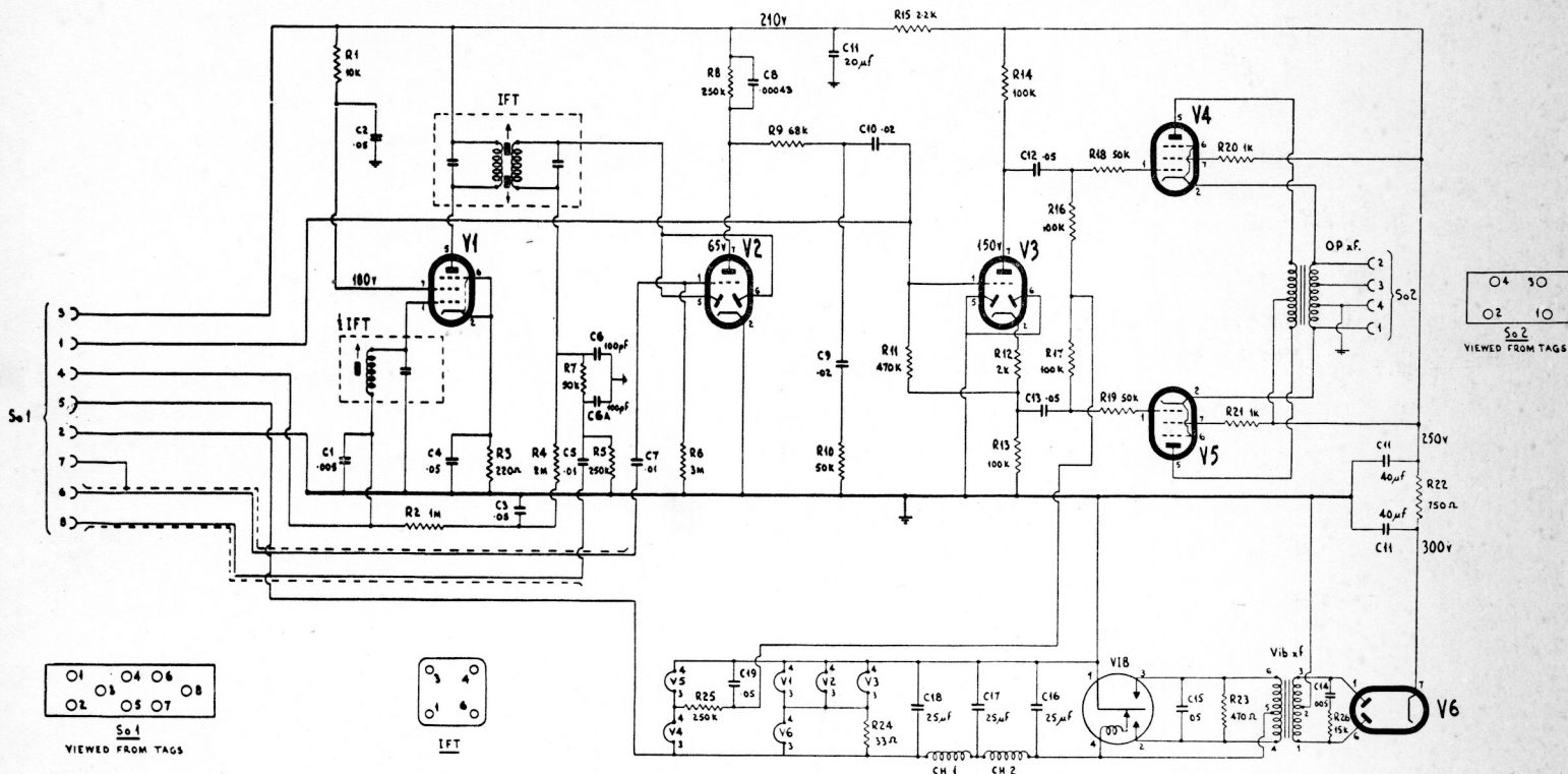
MODEL 536 AMP 8-VALVE RADIOMOBILE AMPLIFIER GBR 7/53.
