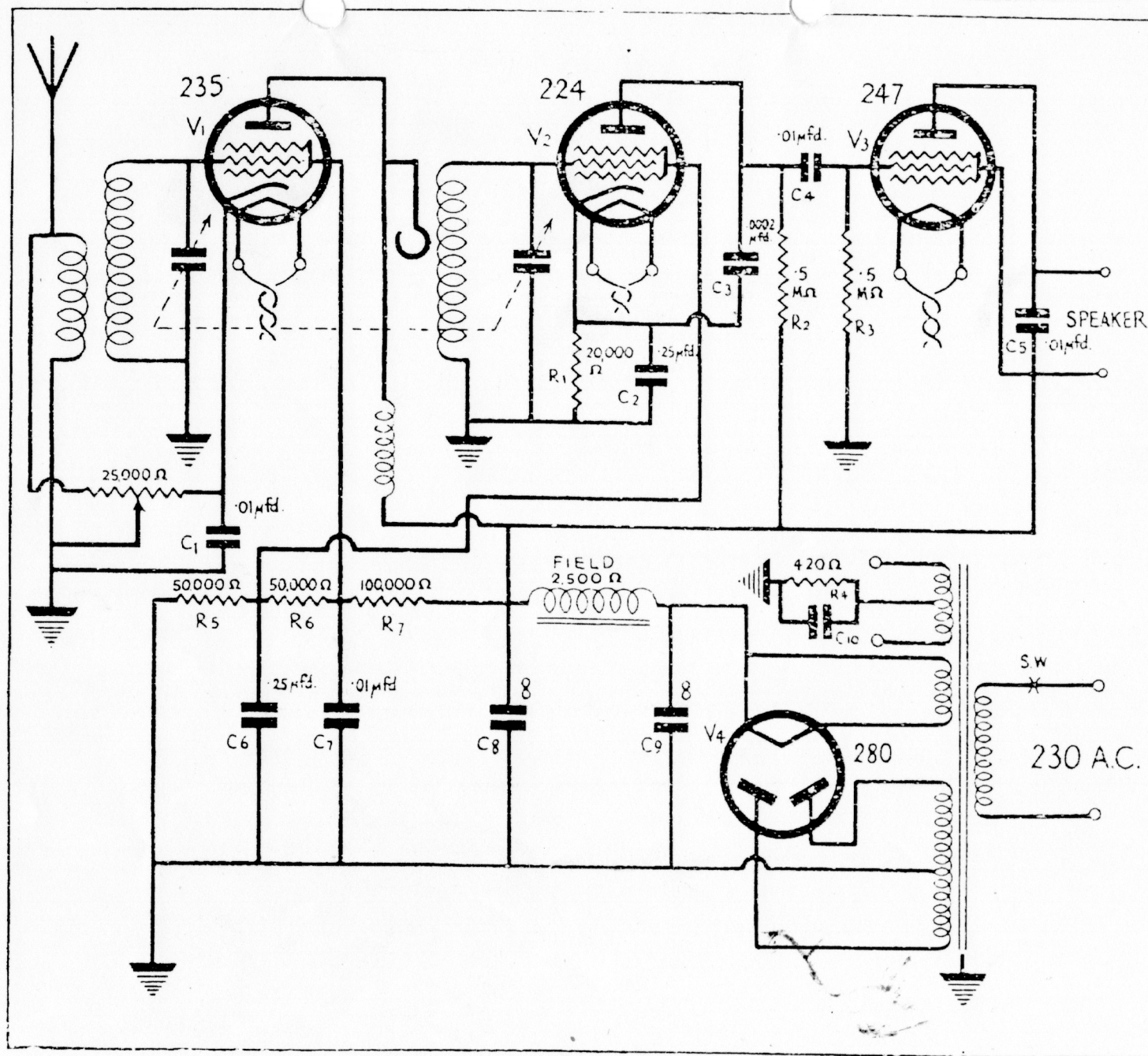
Circuit of the "Kiwi" Four.
