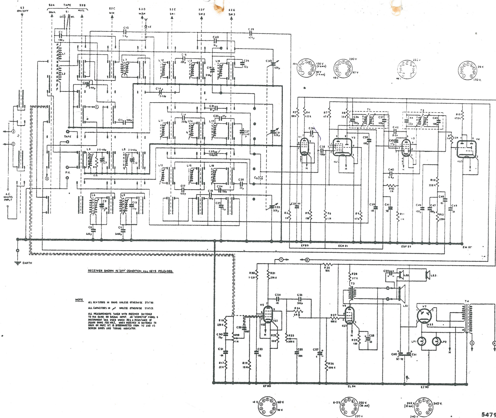
CIRCUIT DIAGRAM of the PYE MODEL P7 340
