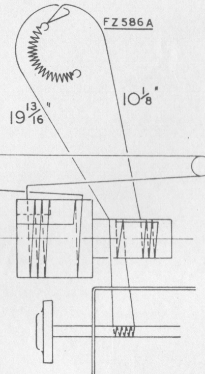
DRIVE CORD ASSEMBLY VK 448-17
