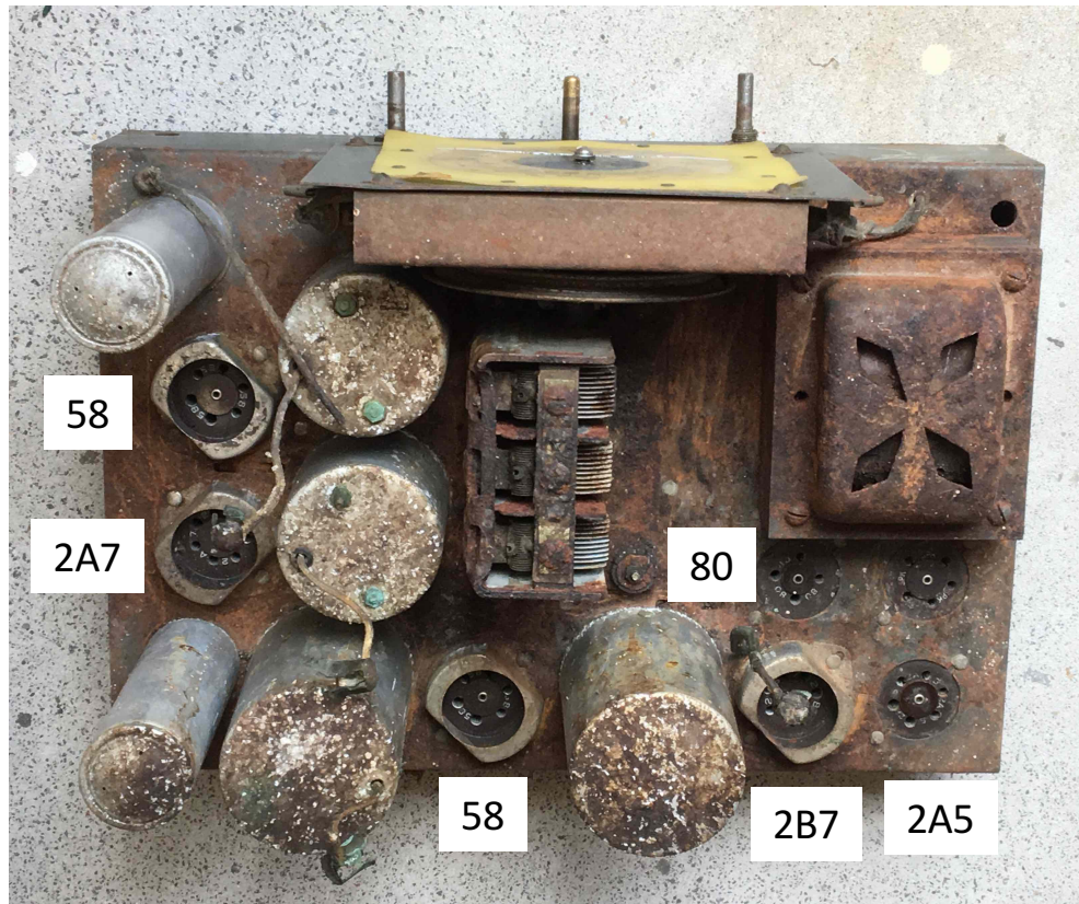
Radio (1936) Ltd Skyscraper model ACS
