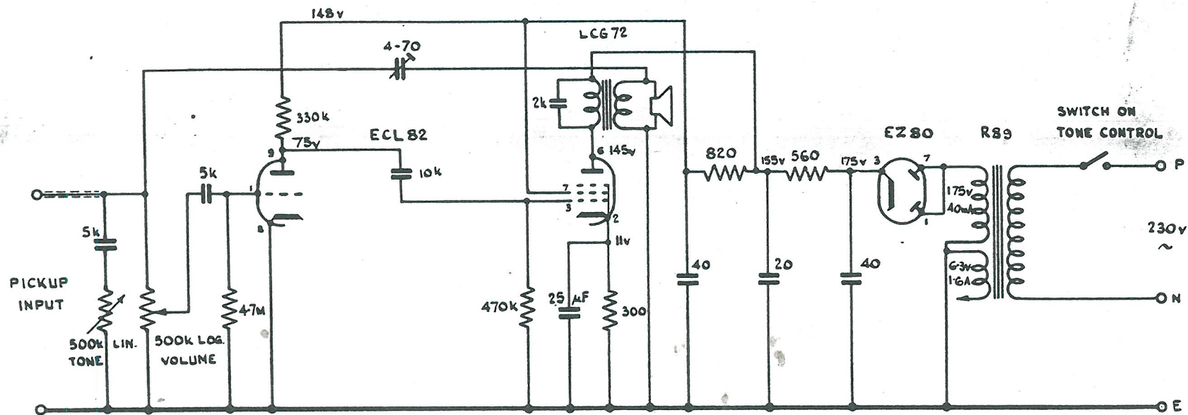
"MAJORETTE" CIRCUIT DIAGRAM
