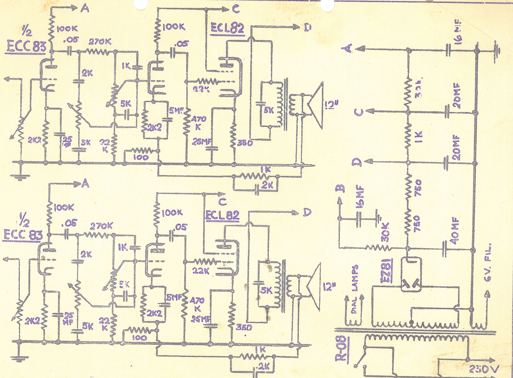
7B61-A AUDIO SECTION & POWER SUPPLY BELL RADIO-TV. CORP LTD.
