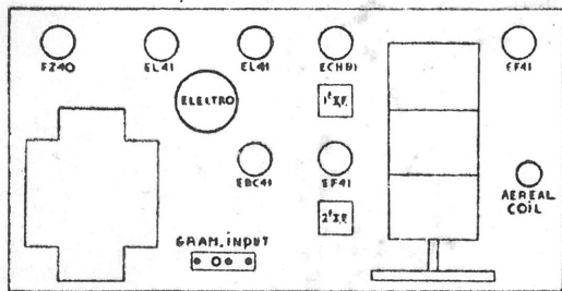
LAYOUT OF TUBES.
