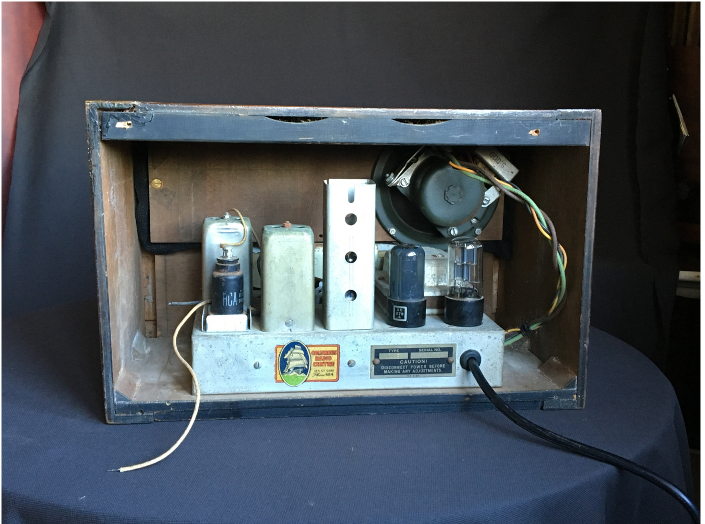
Pacemaker model 516. The circuit is the same as model 515D. Photos: James Davidson
