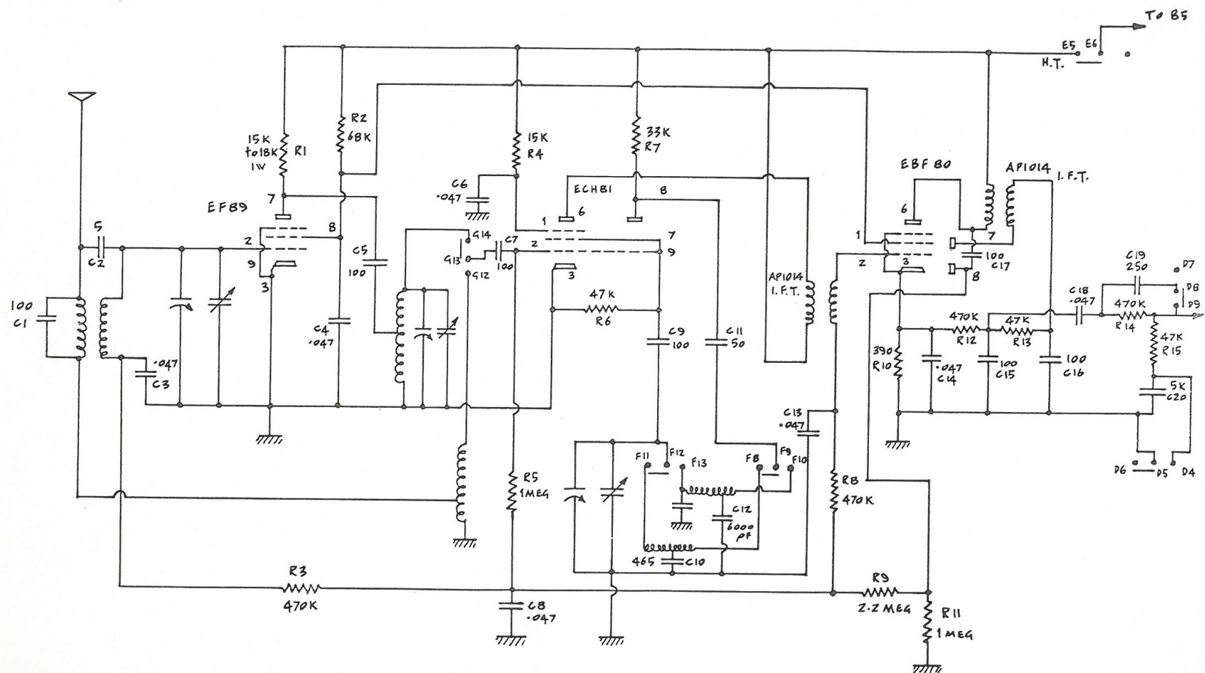
SIX VALVE PUSH-BUTTON DUAL-WAVE.
