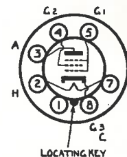
Philco type 41E showing internal resistor.
