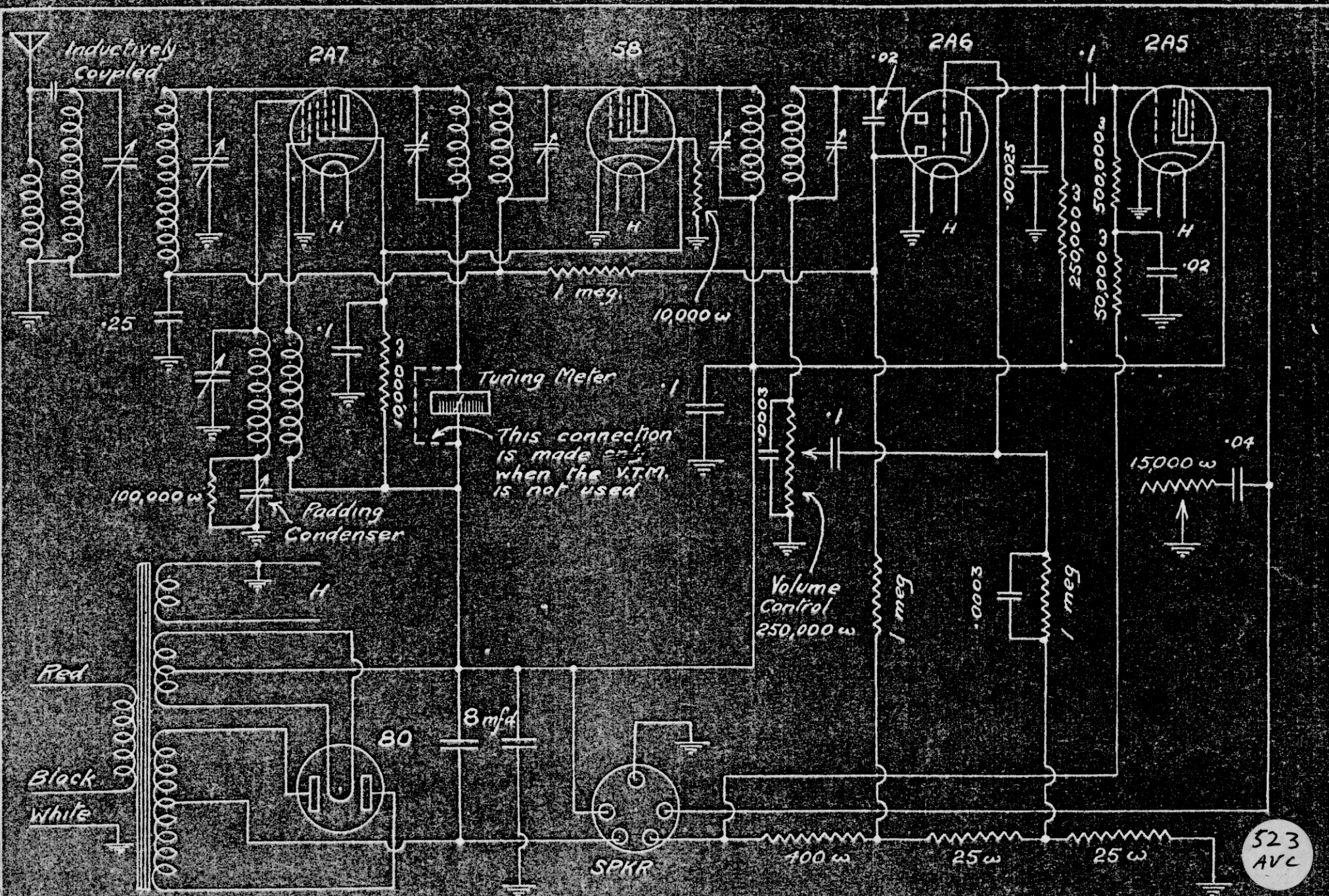
CIRCUIT DIAGRAM OF 5 VALVE A.V.C. RECEIVER.
