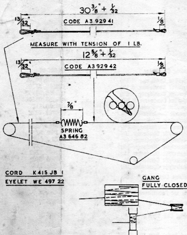
DIAL CORD DIAGRAM
