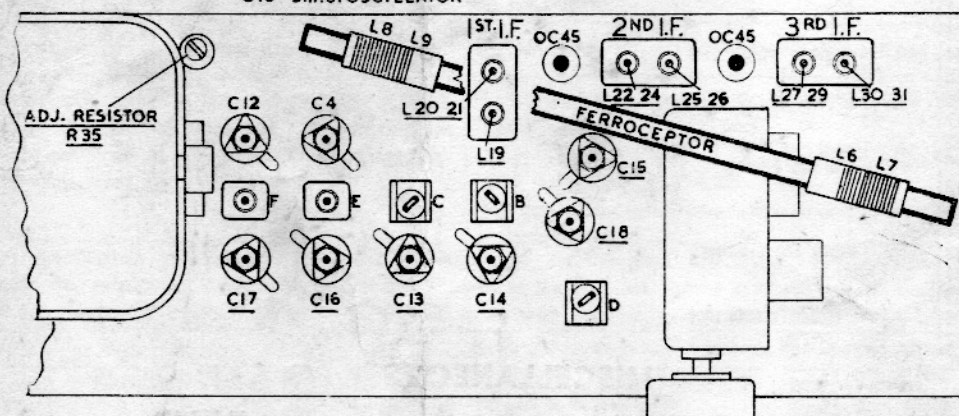
TRIMMER LOCATION DIAGRAM
