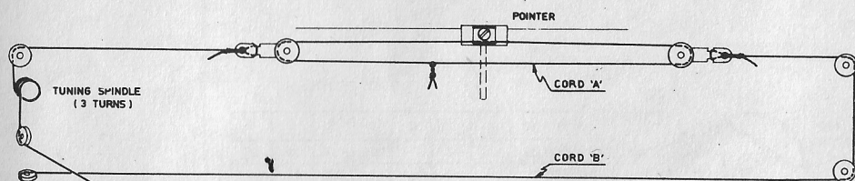
DIAL CORD STRINGING
