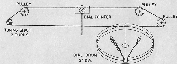
DIAL CORD STRINGING
