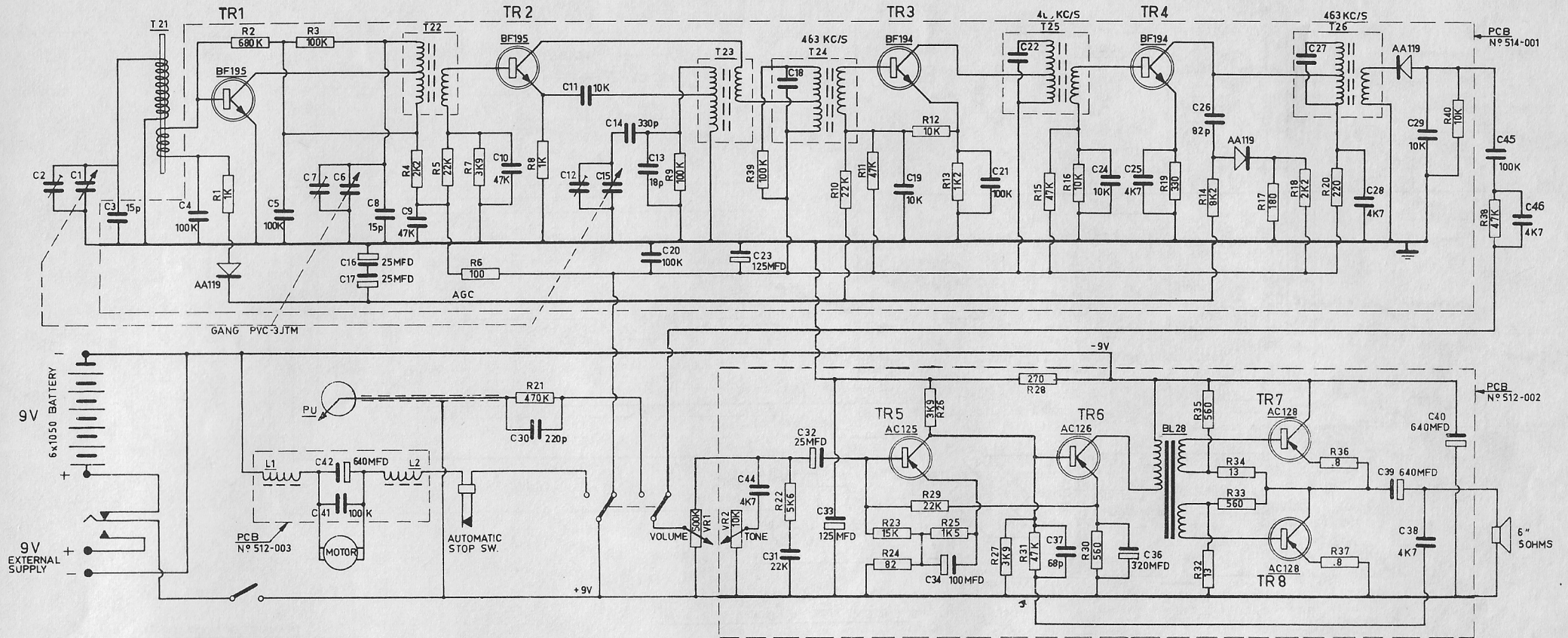
CIRCUIT DIAGRAM
