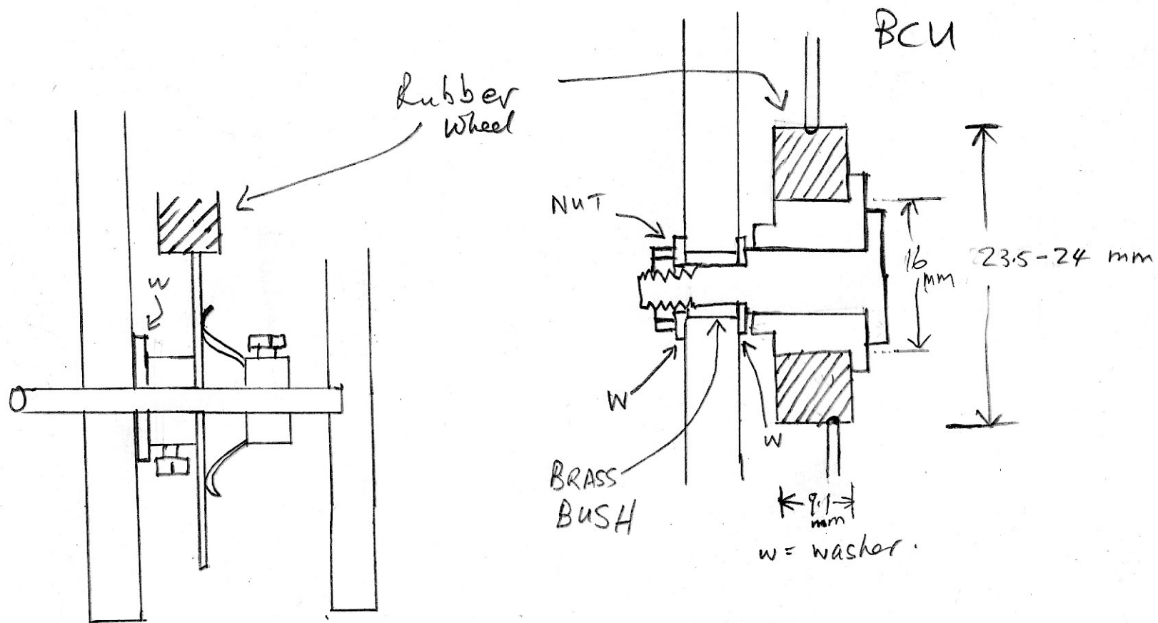
TUNING DRIVE MECHANISM Radio (1936) LTD model BCU
