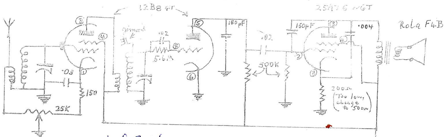
Circuit of 2nd Model.
