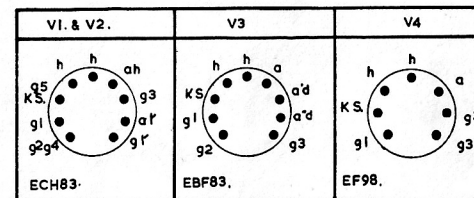
VIEWED FROM UNDERSIDE.
