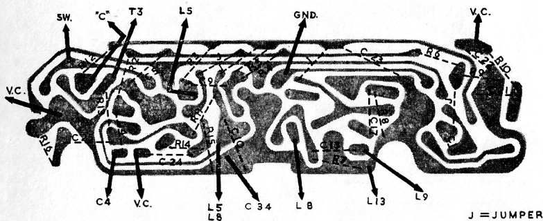
VIEW LOOKING AT COPPER SURFACE
