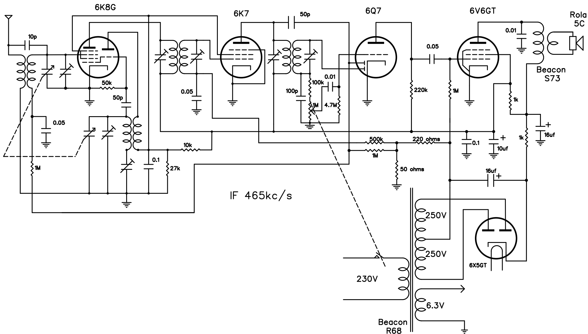
STOKODYNE Circuit (taken from a set)
